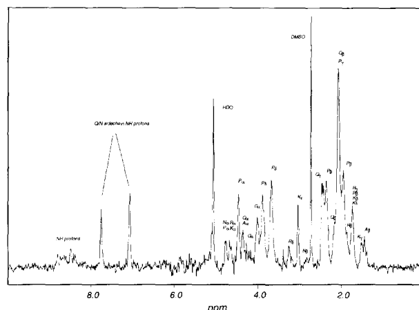
Fig. 1. One-dimensional ^1\text{H} -NMR spectrum of the purified basic PRP. Proton resonances have been labelled with the one-letter amino acid code and carbon atom position.
